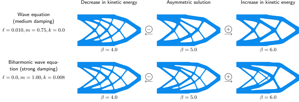
Figure 18: Transition to symmetrical layout by varying parameter \beta .
